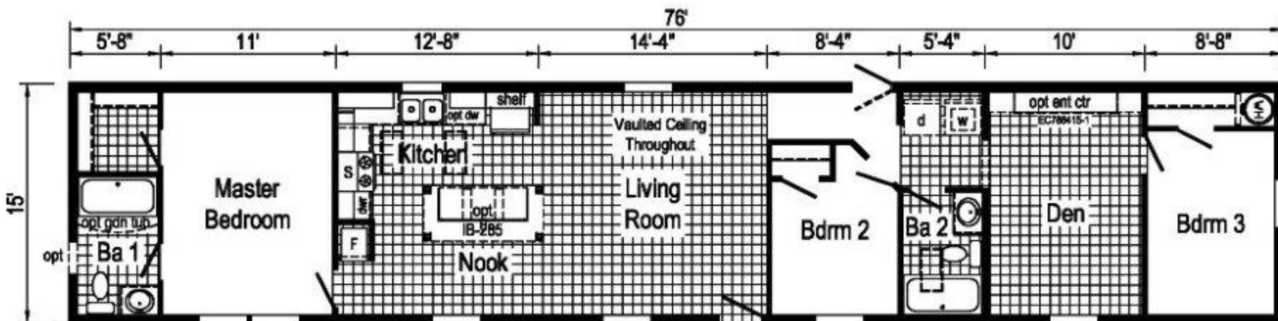
TT110-A 1676 Approx. 1140 Sq. Ft.
